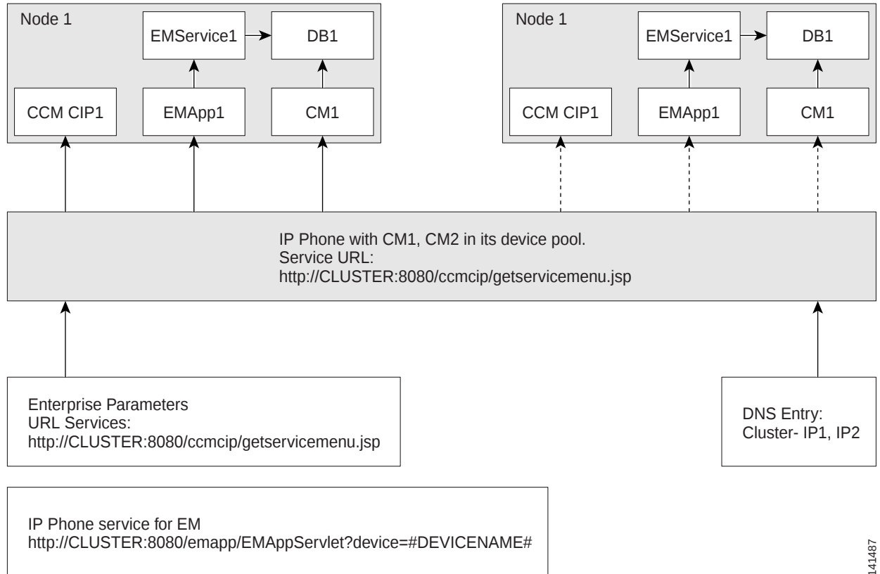
Figure 3-3 Cisco Unified CallManager Extension Mobility Failover Support Components
